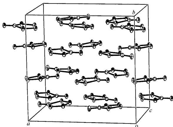
Figure 3. Crystal structure and packing of Roesky's ketone ( 1 )
