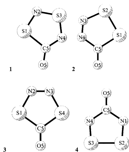
Figure 1. Molecular structure of Roesky's ketone ( 1 ) and its three constitutional isomers (see text for details); note that the numbering of the isomers is not systematic, but conforms to that of the parent compound for clarity
