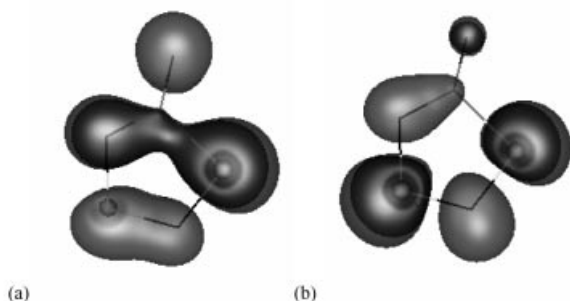
Figure 4. (a) HOMO and (b) LUMO of 5-oxo-1,3,2,4-dithiadiazole ( 1 ); see text for details
