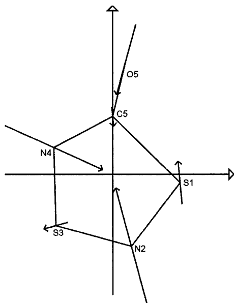
Figure 5. Atomic dipole moments in the Cartesian frame of the calculation; the size of the atomic dipole moment vector arrows has been increased by a factor of 100
