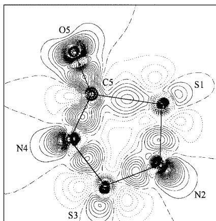
Figure 6. Deformation electron density of Roesky's ketone ( 1 ) in the molecular plane; full lines indicate positive electron density, dashed lines negative electron density and dashed-dotted lines zero electron density; isodensity lines were plotted every 0.05 \text{ e} \cdot \text{Å}^{-3}
